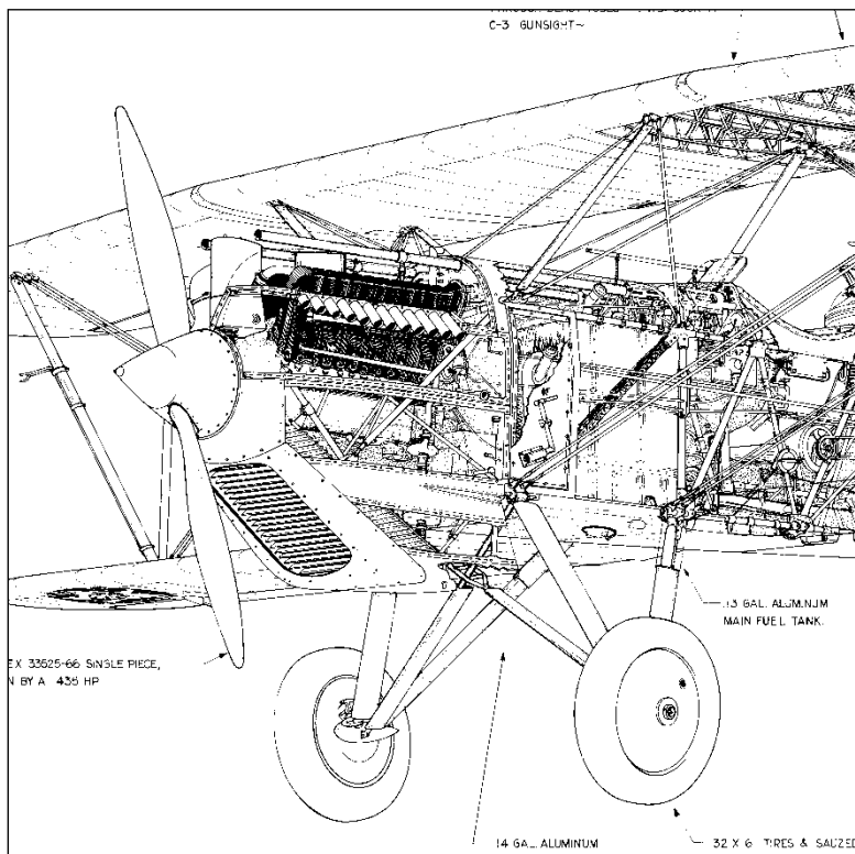
Detail reduced from Nicholas Karstens' drawing of the Curtiss A-3 Falcon.
